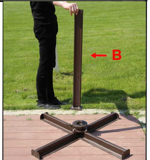
Step2. Place the rotating device (L) onto the cross base with 4 bolts (H). Tighten bolts with Part (I). Place the tube (B) onto the rotating device (L).
