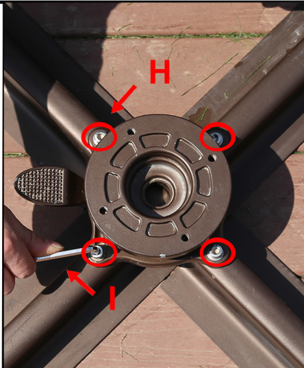
Step2. Place the rotating device (L) onto the cross base with 4 bolts (H). Tighten bolts with Part (I). Place the tube (B) onto the rotating device (L).
