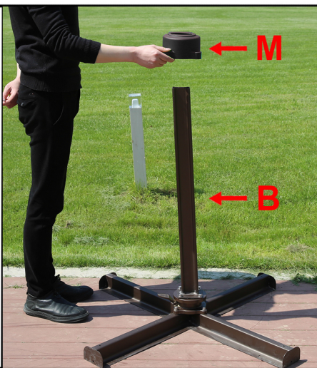
Step3. Connect the two parts with 4 bolts (G). Place Part (M) on the tube (B).
