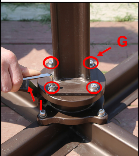
Step3. Connect the two parts with 4 bolts (G). Place Part (M) on the tube (B).
